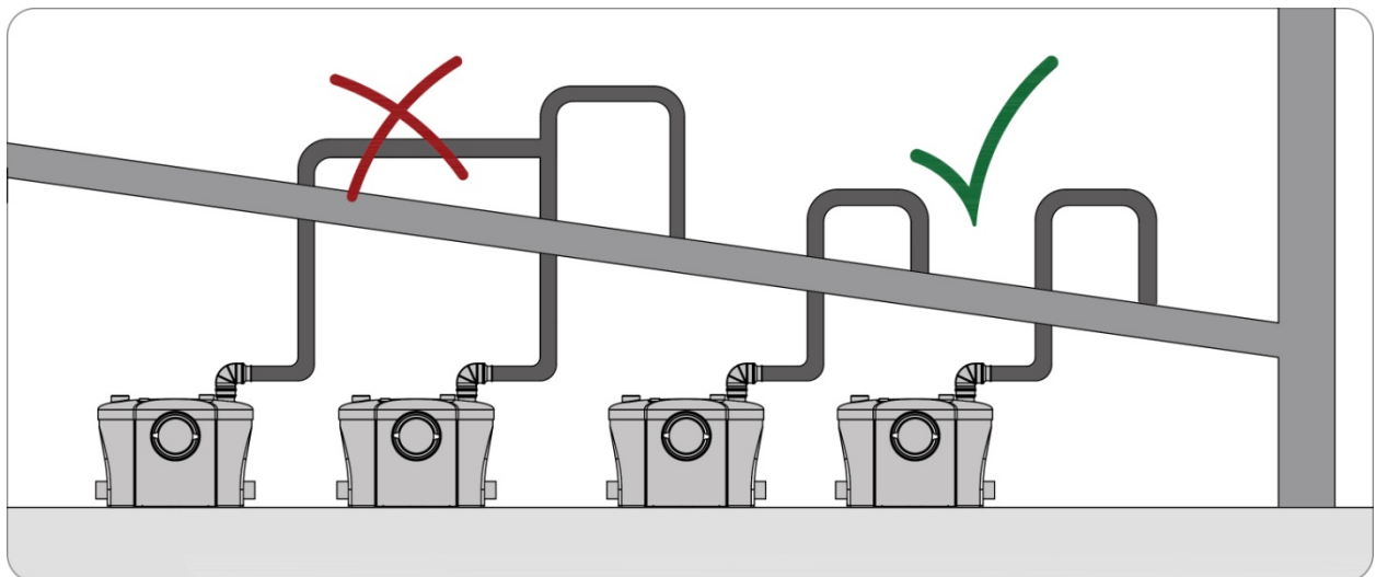
Fig14&15: Discharge Pipe connection
