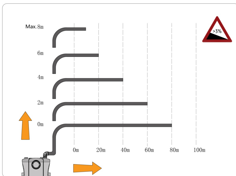
Fig10: Pumping head
