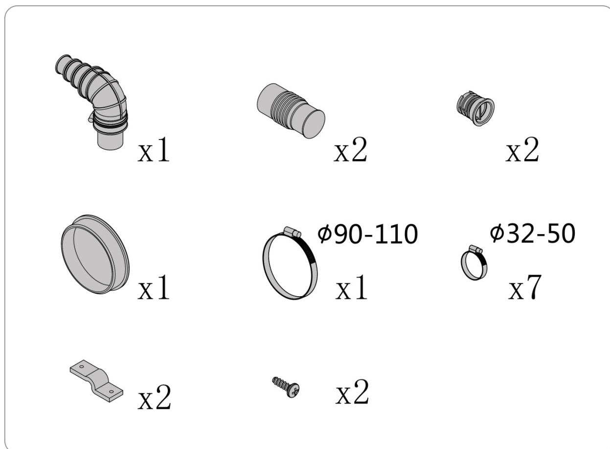
Fig2: Spare parts
