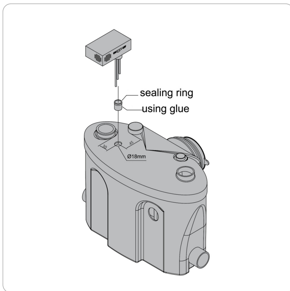
Fig10: Pumping head
