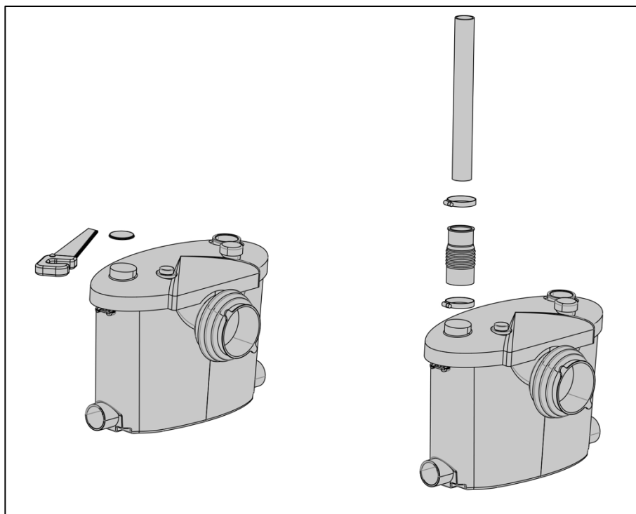
Fig8: Outlet (Check Valve)
