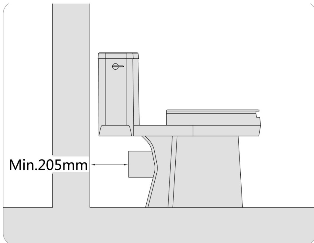
Fig12: Min Size from toilet outlet to rear wall is 205mm
