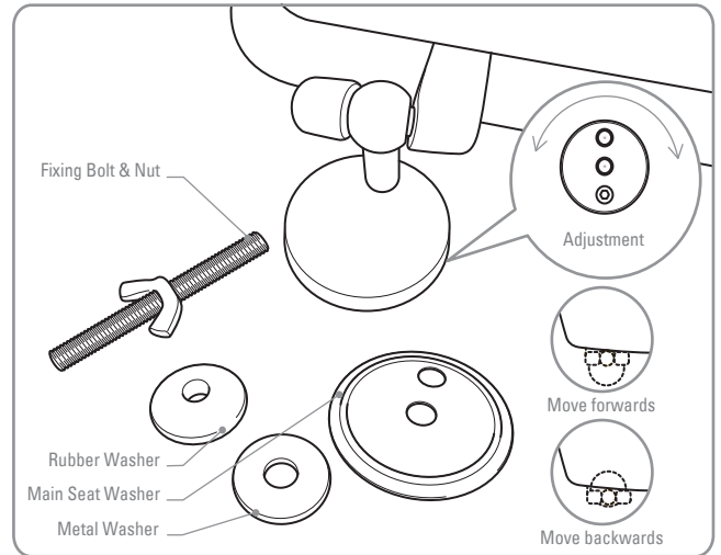
PARTS DIAGRAM
