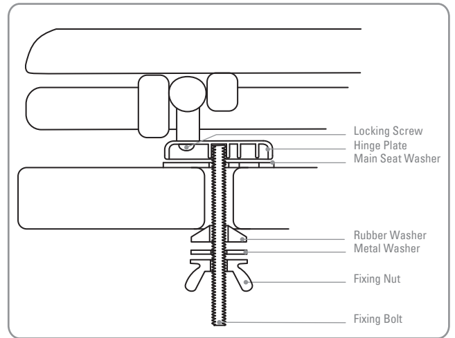
ASSEMBLY DIAGRAM
