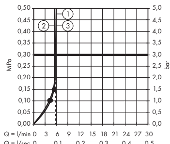
Croma 100 Multi 26830000
