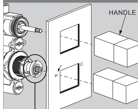
FIG. 2 FITTING CONTROL HANDLES
