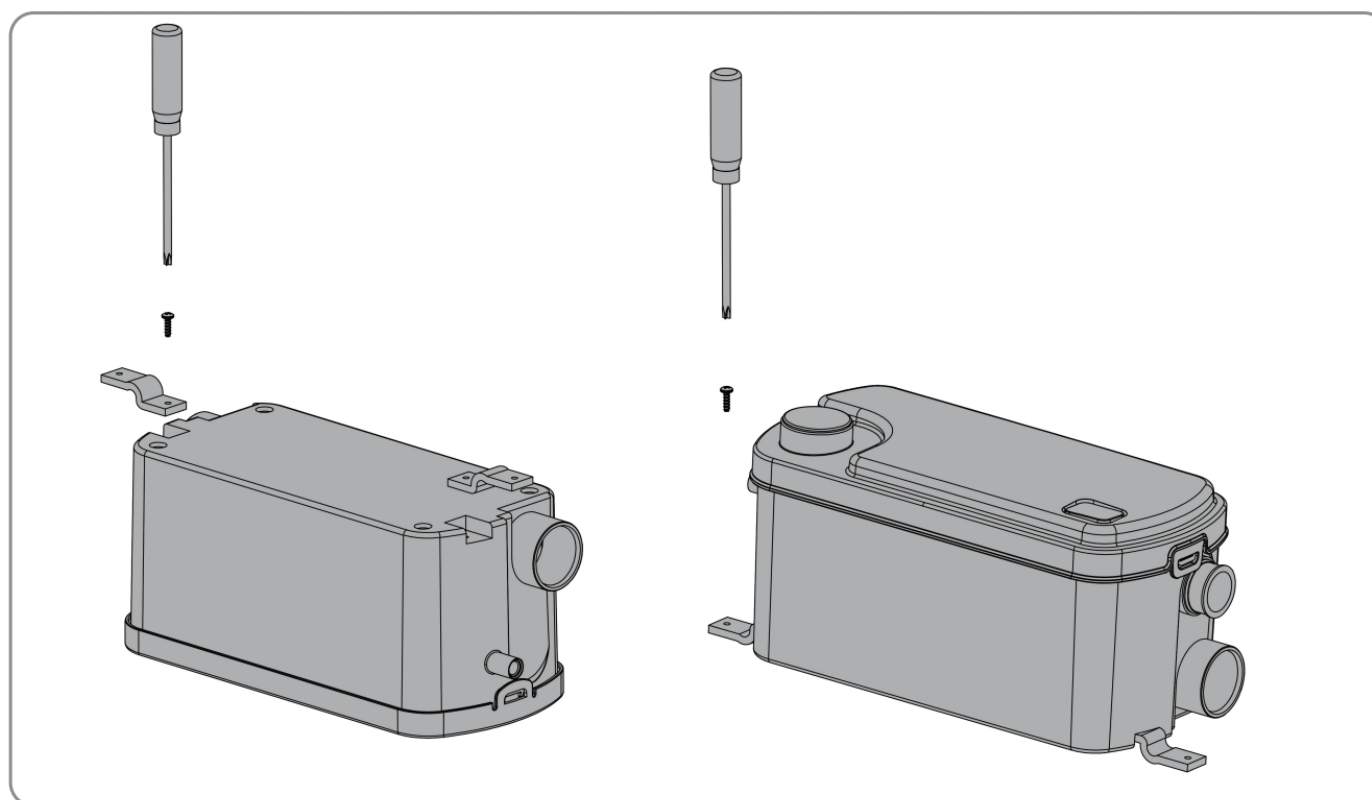
Fig6: Fixation
