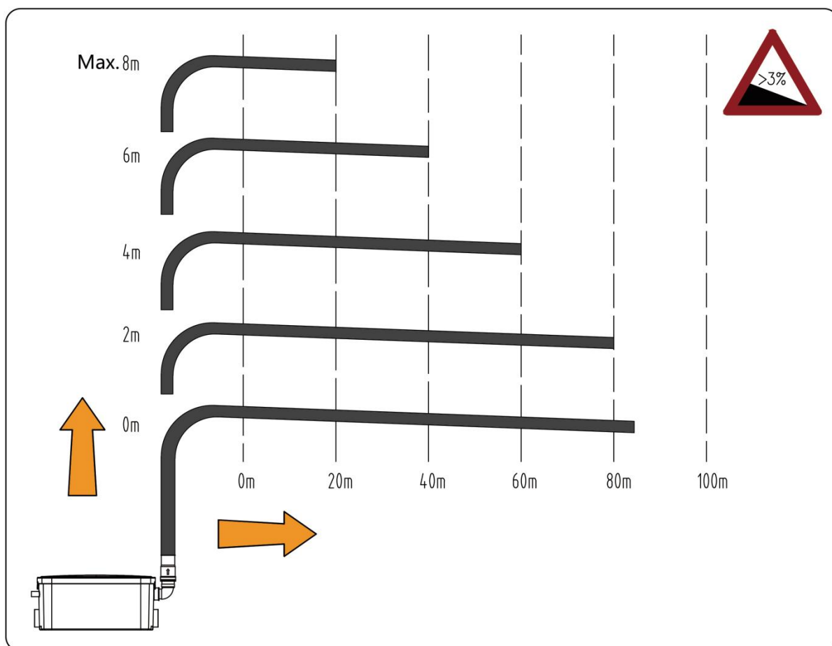
Fig8: Pumping head
