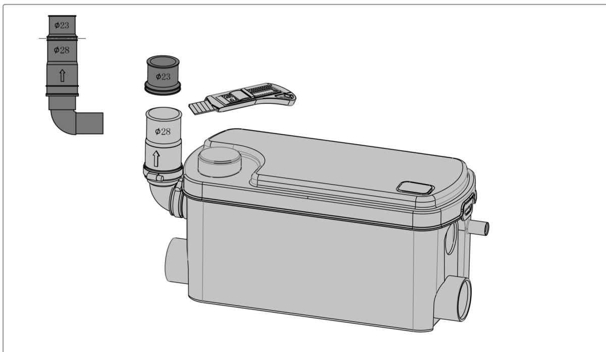
Fig8: Pumping head
