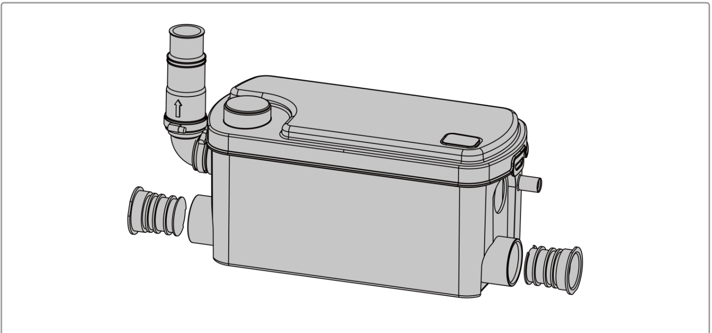
Fig4: Connection
