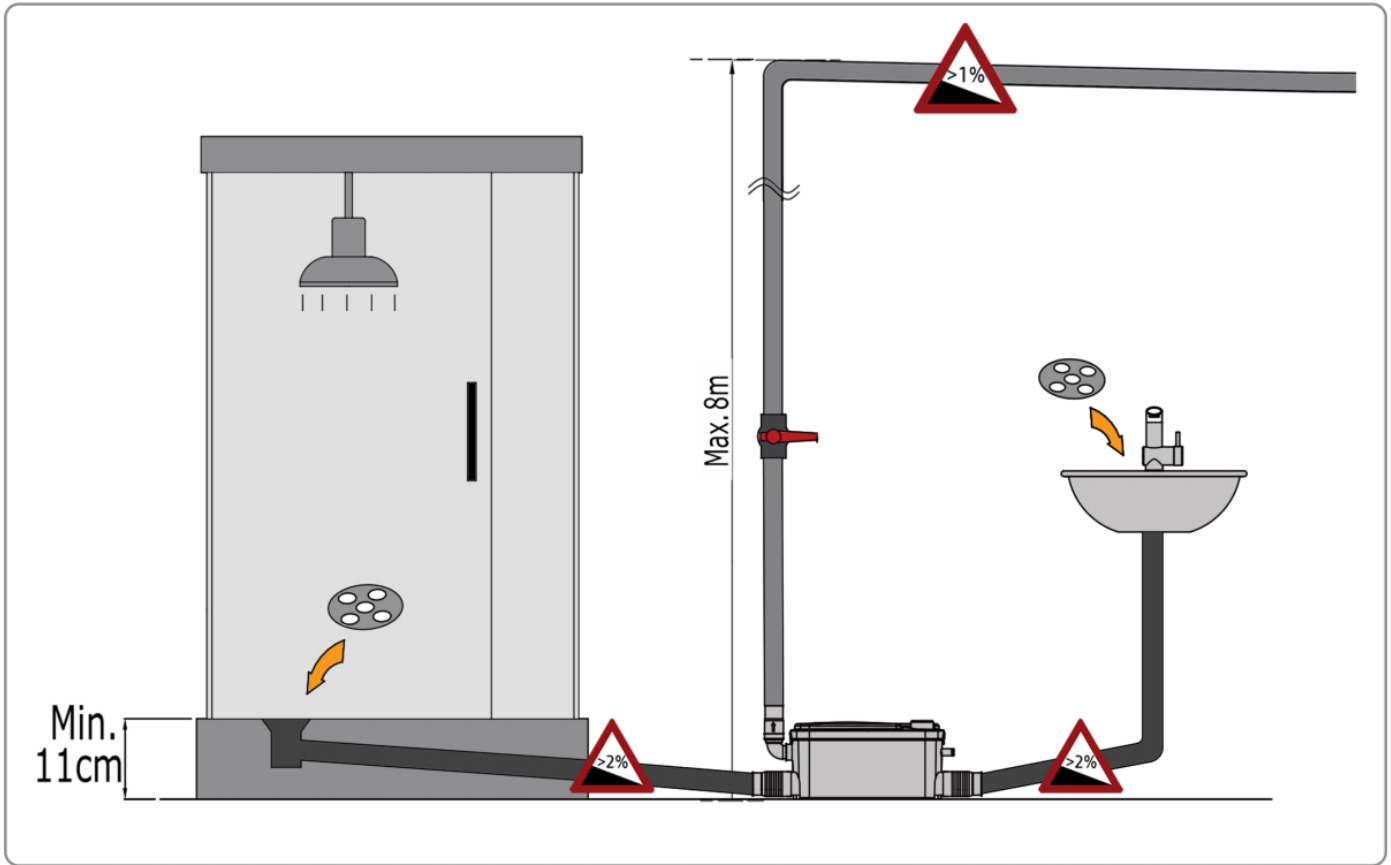
Fig4: Connection
