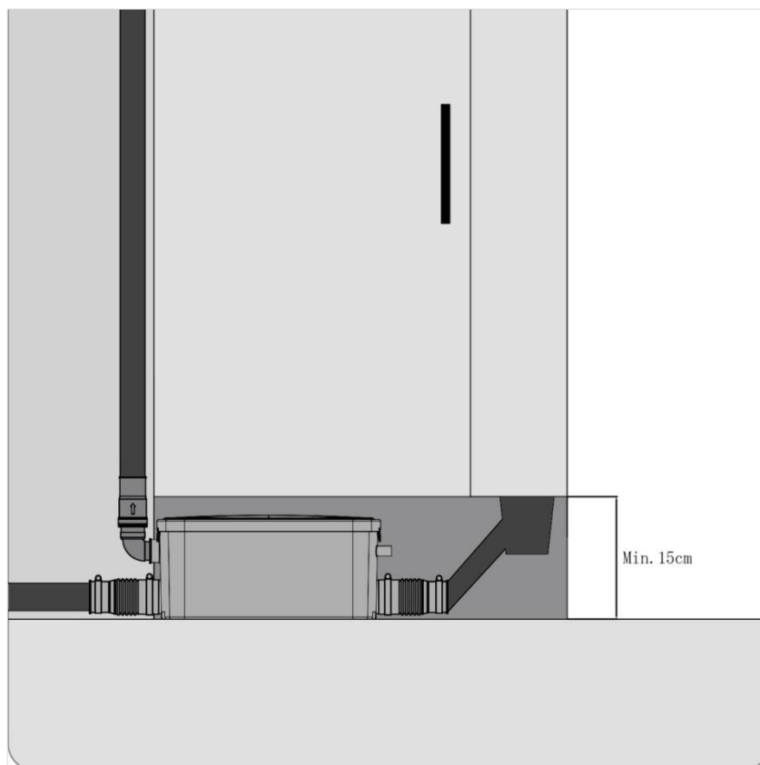
Fig10: Min Size below the shower is 150mm
