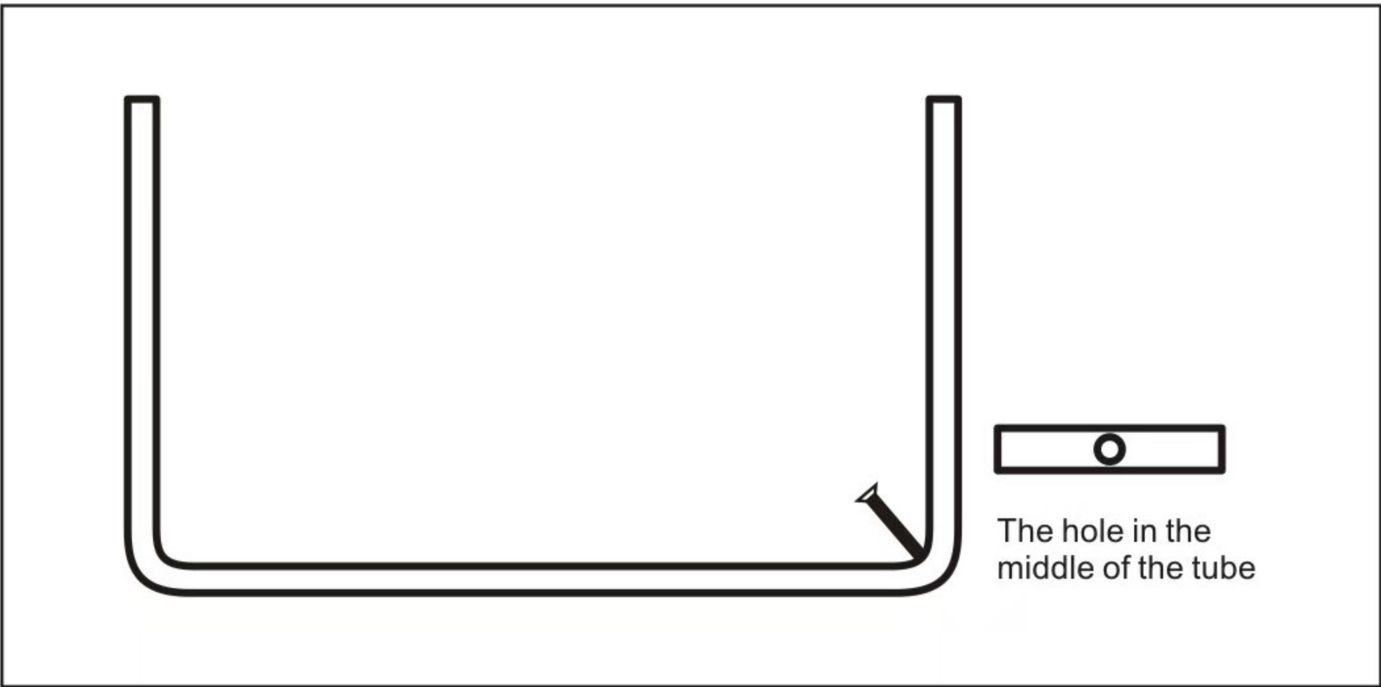
4.Connect the bottom support to the tubes (middle ) with the long screws .
