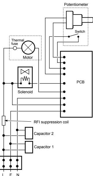
Fig.4 (schematic view)
