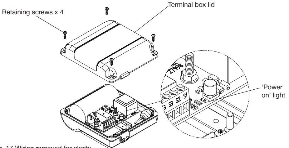
Fig. 17 Wiring removed for clarity
