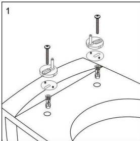
Insert the hinges into the toilet.
