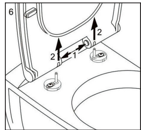
Take off the toilet seat by pressing both push buttons.
